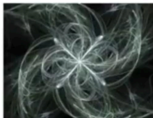
Electron Clouds
