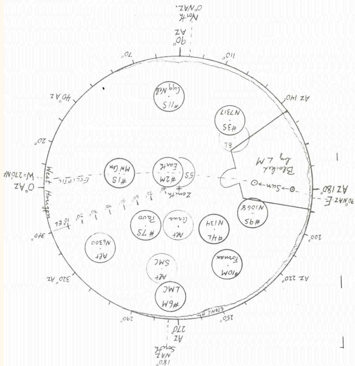
Fig. 8 April Target Pointing (Outside View of Descartes' Celestial Sphere)
