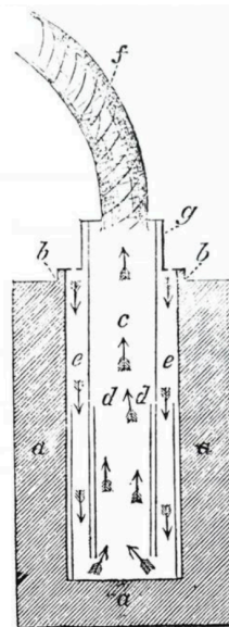
Perpendicular section of inhaler on a scale of one-half the dimensions.
